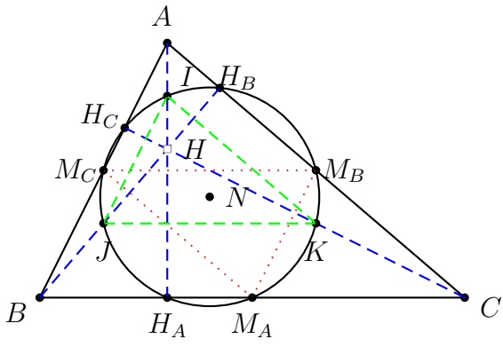
Figure 1: Euler-Feuerbach Circle.
