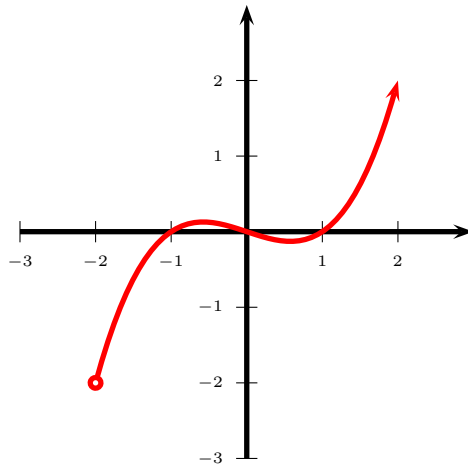
Figure 1: Graph of x \mapsto \frac{x^3 - x}{3} .
